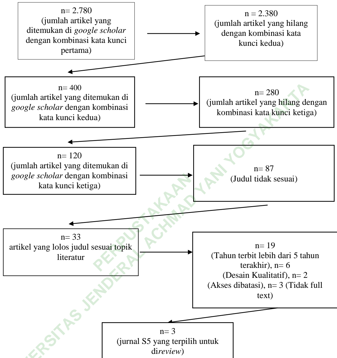
Bagan 3. 1 Flowchart
