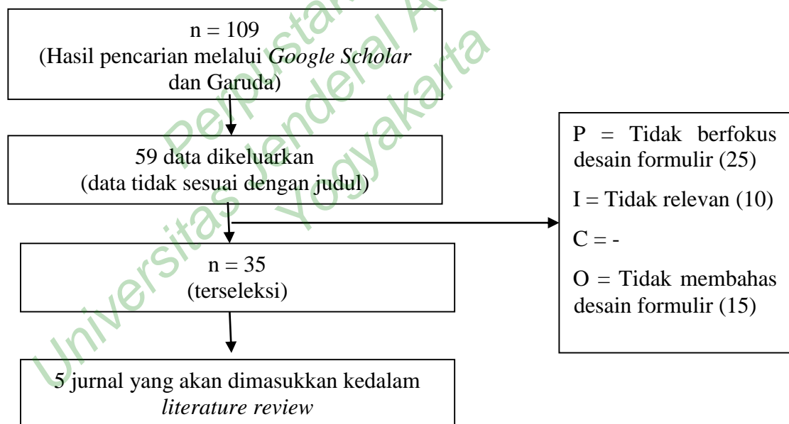
Gambar 3. 1 Pencarian Jurnal
