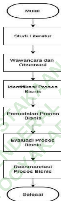
Gambar 3. 1 Alur Penelitian
